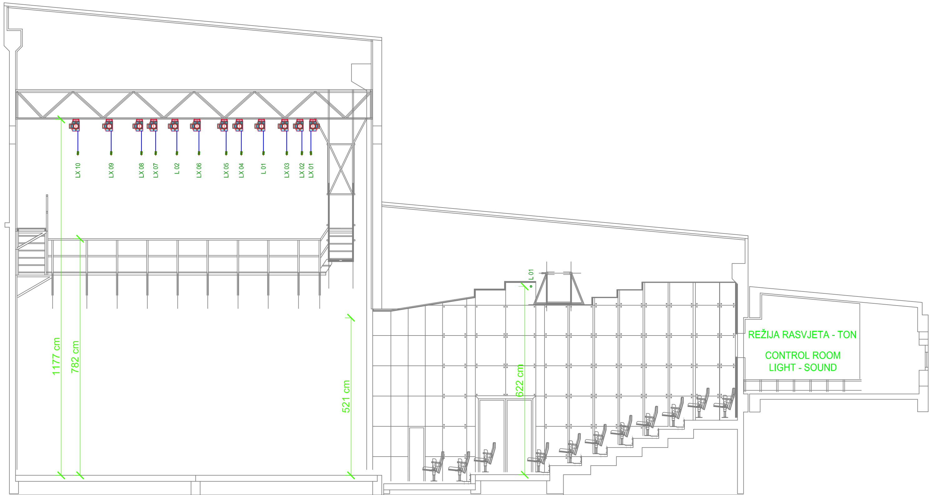
POVLAKE - PRESJEK HOISTS - CROSS SECTION
